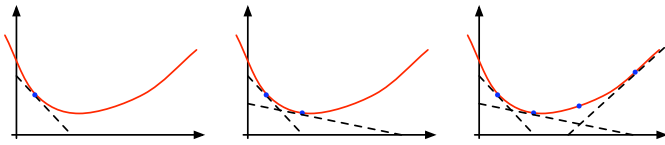
Figure 1: A convex function (solid) is bounded from below by Taylor approximations of first order (dashed). Adding more terms improves the bound.
